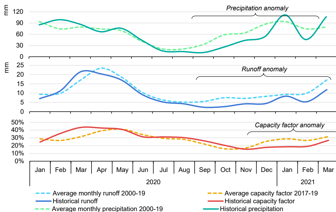
Figure 3.27 Sensitivity of hydropower capacity factors to precipitation and runoff levels, Turkey, 2020-2021
