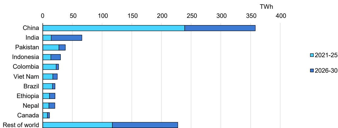
Figure 3.21 Main-case increases in annual gross hydropower generation among top ten countries with largest growth, 2021-2025 and 2026-2030
