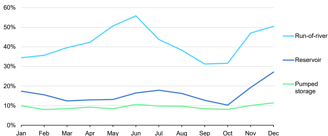
Figure 3.26 Average monthly capacity factor by plant type, selected European countries, 2019
