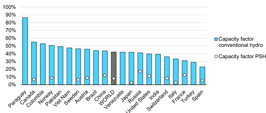
Figure 3.23 Average overall and PSH-specific hydropower capacity factors, world and top 20 generating countries, 2015-2019
