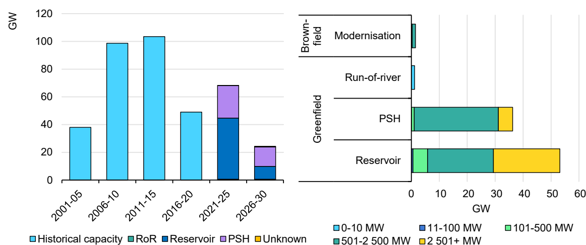
Figure 3.8 China hydropower capacity additions by application, 2000-2030 (left) and by size, 2021-2030 (right)
