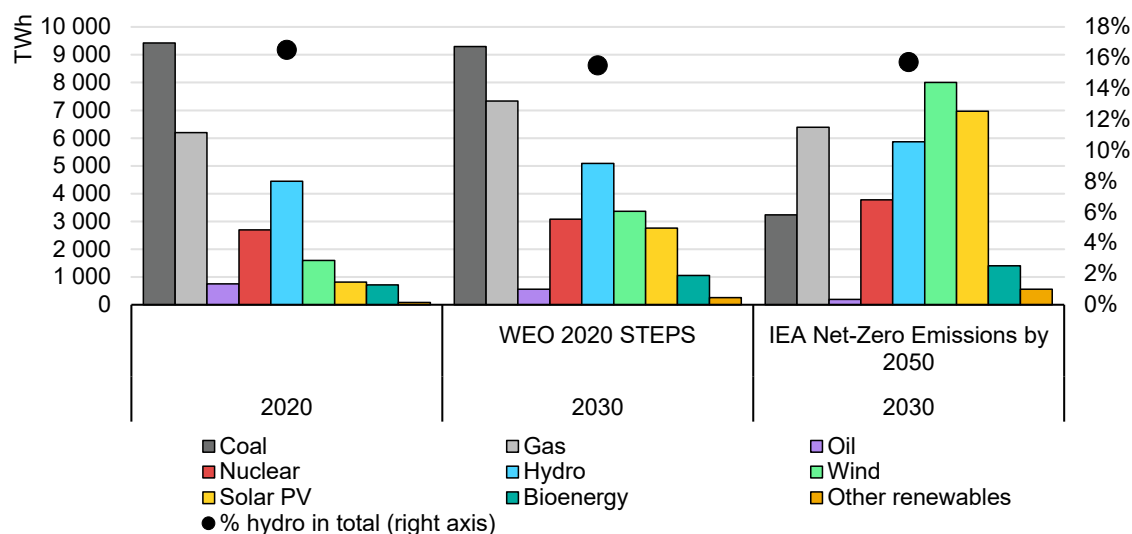
Figure 3.22 Global electricity generation by source in STEPS and SDS, 2020-2030
