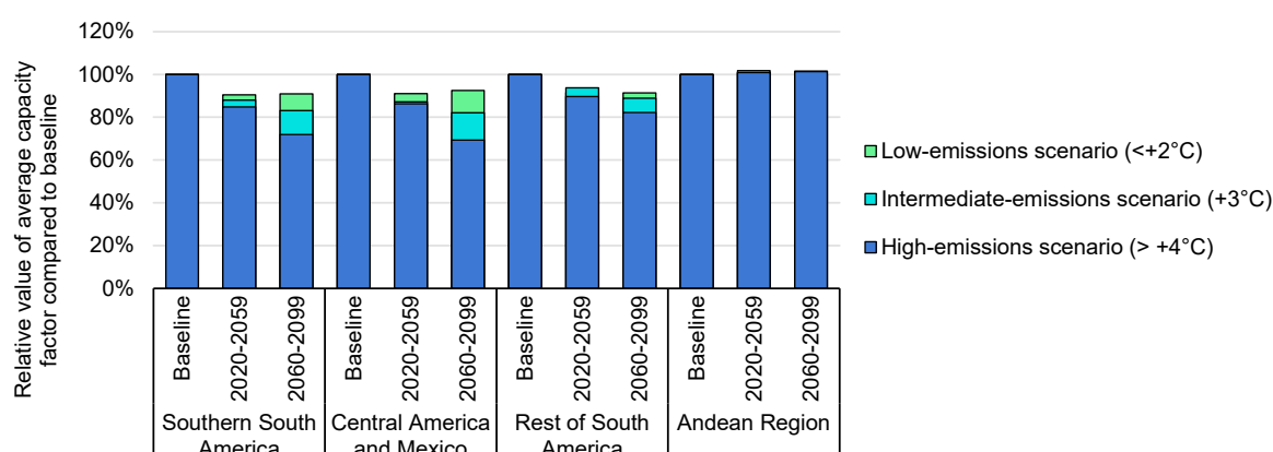
Figure 3.28 Hydropower capacity factor evolution in Latin America, 2020-2099
