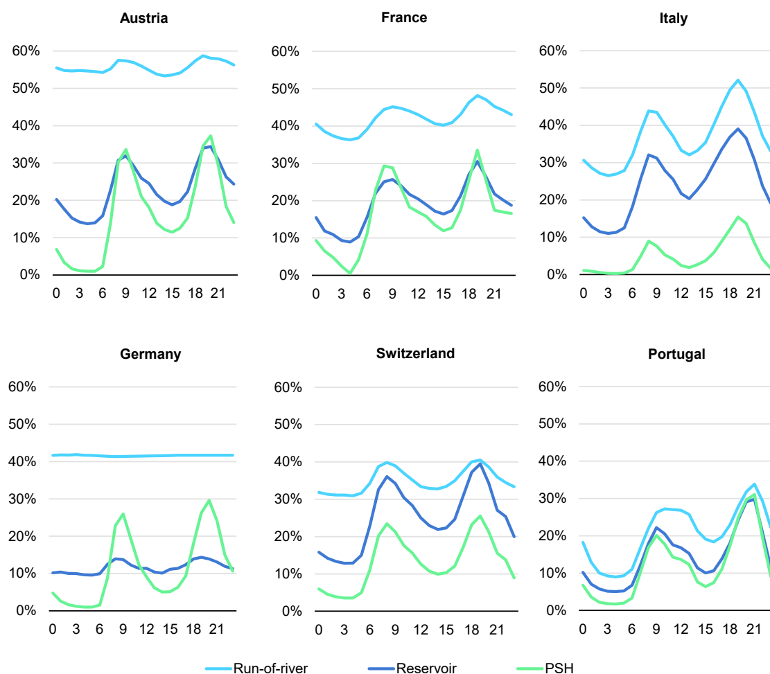
Figure 3.24 Annual average run-of-river, reservoir and PSH generation capacity factors for one day in selected countries, 2019
