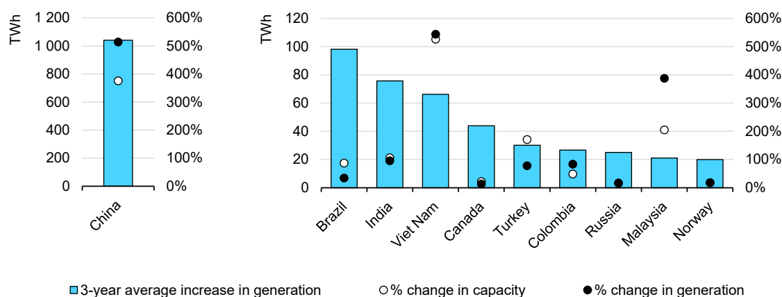
Figure 3.20 Gross hydropower generation and capacity growth among top ten countries with largest increases, 2000-2019
