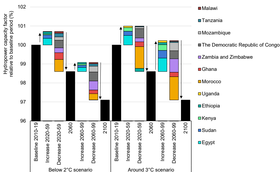
Figure 3.29 Hydropower capacity factor evolution in Africa, 2020-2099
