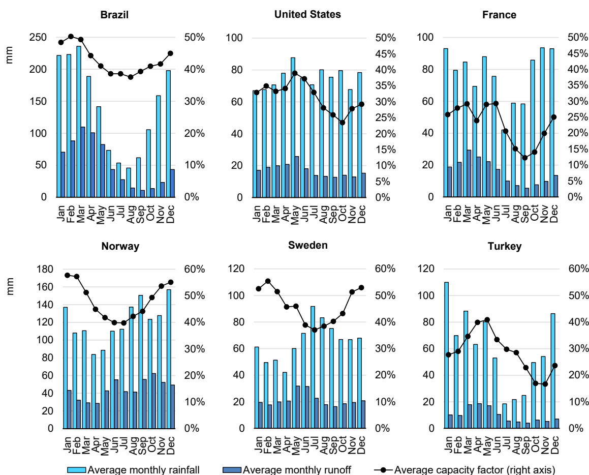
Figure 3.25 Average monthly rainfall, runoff and hydropower capacity factors for selected countries, 2015-2020 and 2017-2020
